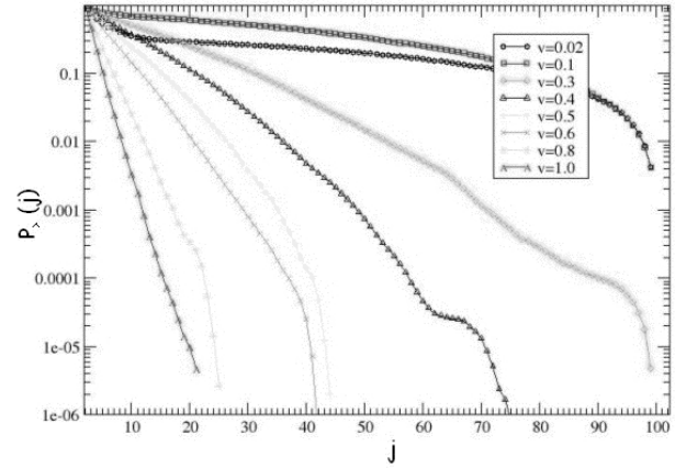
Fig. 12 Cumulative distribution functions of the jam-size values, for various drag velocities, v . Please note the log-normal scales.
